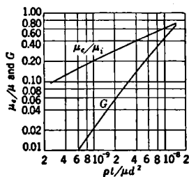
FIG. 15-20.—Plot of \frac{\mu_e}{\mu} and the eddy-current loss during and after the pulse [that is, Terms 1 and 3a of Eq. (27), or the energy W_e represented by area e in Fig. 15-18].
